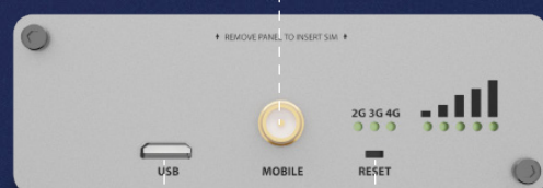
USB connector
