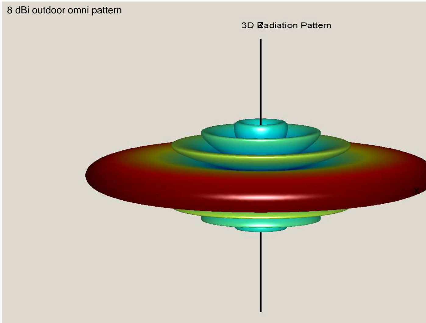
Figure 6. Radiation pattern of an omni-directional antenna
