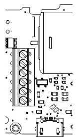
6 - Connect the ends of the meter cable to the screw terminals.
