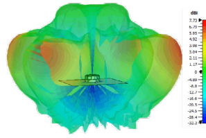
Typical 3D Pattern LTE Elements Side 5400MHz
