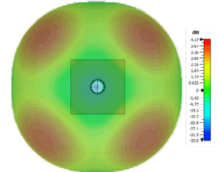
Typical 3D Pattern LTE Elements Top 1800MHz
