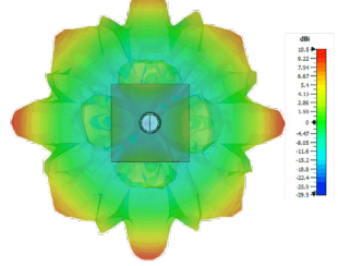
Typical 3D Pattern WiFi Elements Top 5400MHz
