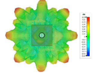
Typical 3D Pattern LTE Elements Top 5400MHz
