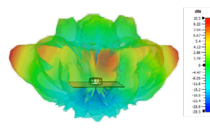
Typical 3D Pattern WiFi Elements Side 5400MHz
