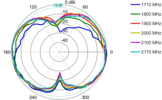
Elevation: 1710 - 2170 MHz
