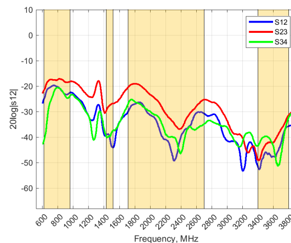
Isolation
