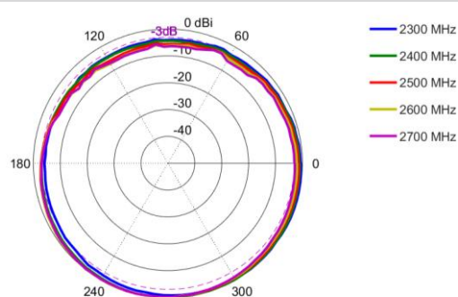
Azimuth: 2300 - 2700 MHz
