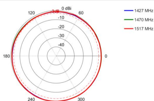
Azimuth: 1427 - 1517 MHz
