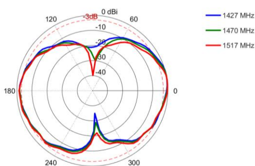
Elevation: 1427 - 1517 MHz
