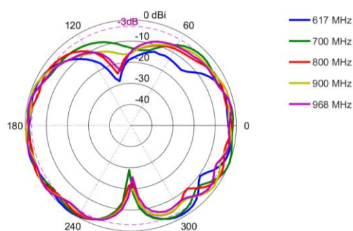
Elevation: 617 - 960 MHz
