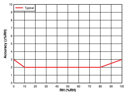
Figure 6-1. RH Accuracy vs. RH
